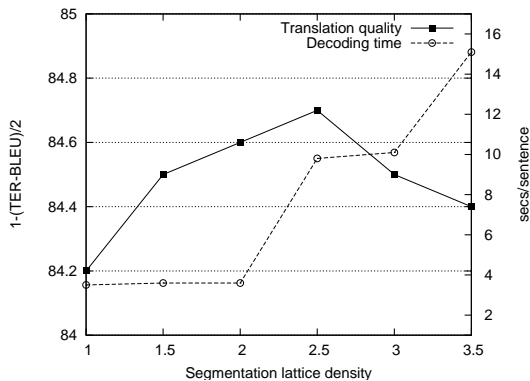
Figure 4: The effect of the lattice density parameter on translation quality and decoding time.
